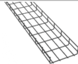
X-Tray 220x60 L=2300 mm | Wire Ø 5
